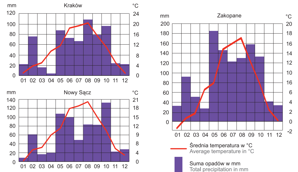
CHART 1. AIR TEMPERATURES AND ATMOSPHERIC PRECIPITATION IN SELECTED METEROLOGICAL STATIONS IN 2020
