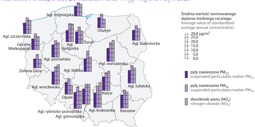
Map 1. Concentration of suspended particulates matter PM_{2.5} , PM_{10} and NO_2 in 2023
