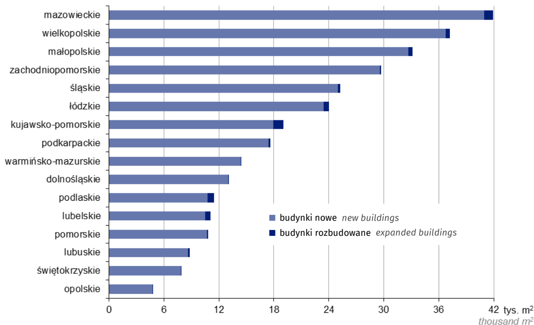
Chart 25. Useful floor area of traffic and communication buildings completed in 2024 by voivodships
