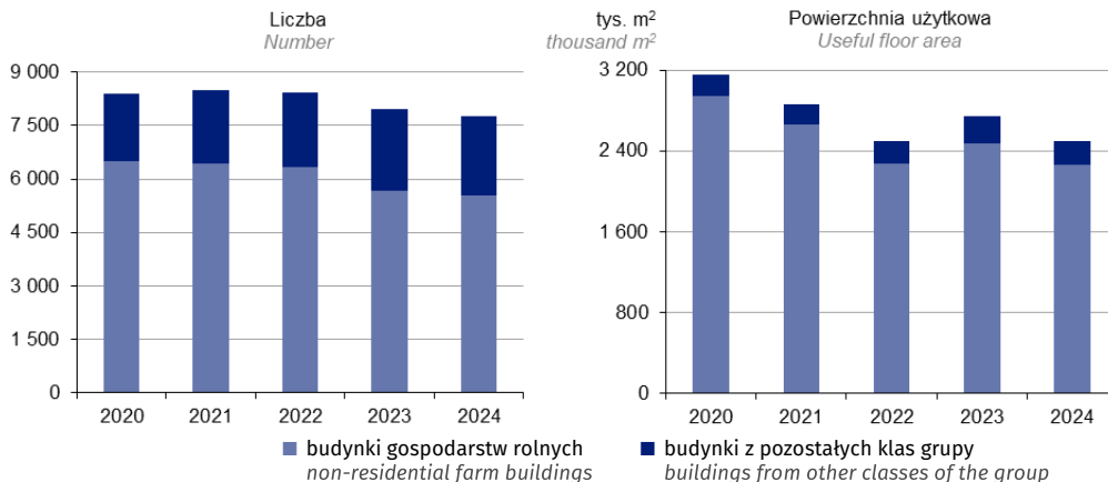
Chart 34. Number and useful floor area of other non-residential buildings completed in 2020-2024
