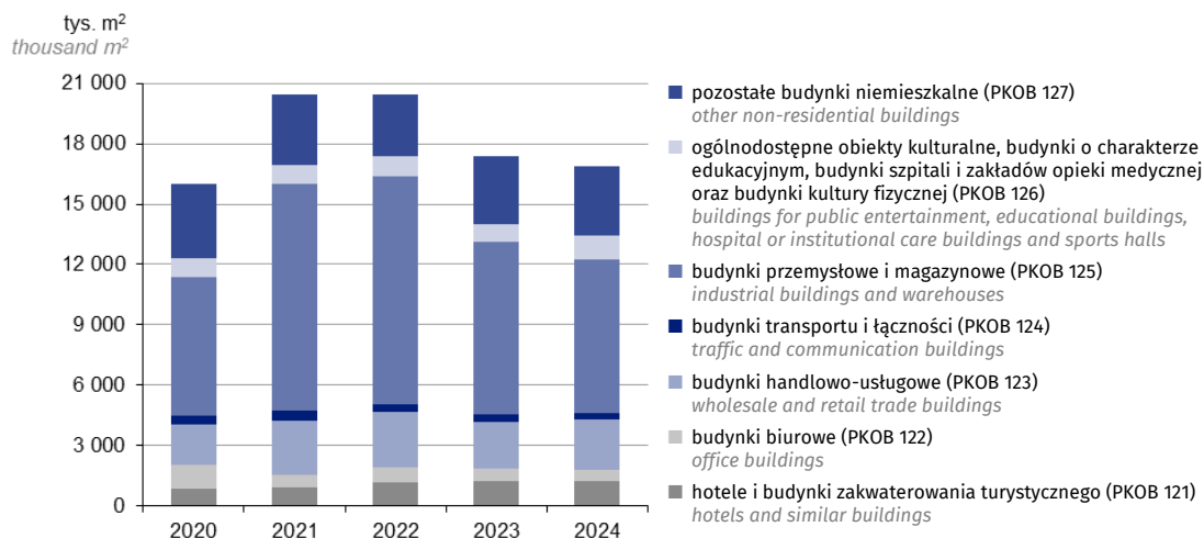
Chart 36. Useful floor area of non-residential buildings for which permits have been granted in 2020-2024 by groups of PKOB
